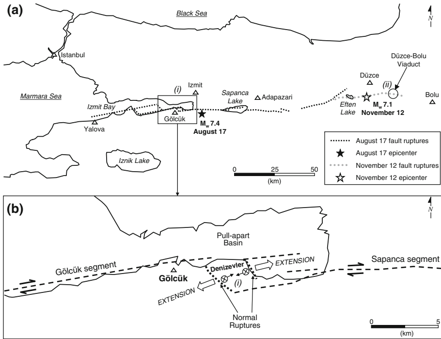
Fig. 1 a Surface fault ruptures of the Turkey 1999 Mw 7.4 Kocaeli (August 17) and Mw 7.1 Düzce (November 12) Earthquakes, along with the two areas of interest: (i) Denizzeveler, east of Gölcük, (ii) the Düzce-Bolu Viaduct; b the step-over mechanism responsible for the normal fault ruptures that passed through Denizzeveler (based on Youd et al. 2000)
