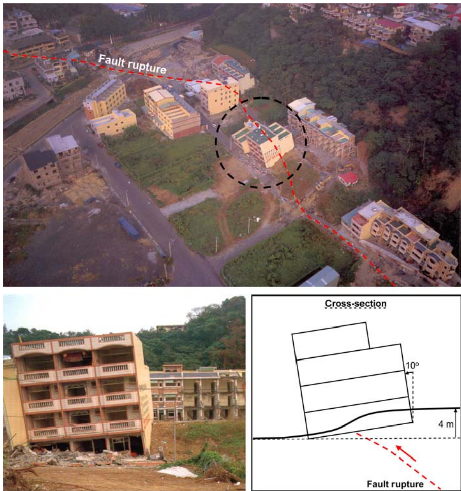
Fig. 7 Chelungpu thrust fault, Chi-Chi, Taiwan 1999 earthquake—Chung-Cheng Park, Fung-Yan City: 4-story building resting on a continuous and rigid foundation (photos adapted from Hwang 2000 ). The building survived 4 m of upthrust without substantial structural damage, but subjected to approximately 10^\circ of rigid-body rotation
