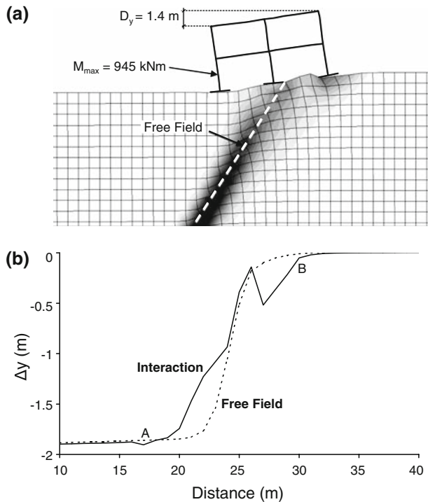
Fig. 16 Normal fault east of Gölcük, Kocaeli, Turkey 1999 earthquake—Denizevler—2-D finite element analysis of the Mosque, Fig. 14a ( h = 2 m): a Deformed mesh and plastic strain, b Vertical displacement \Delta y at the ground surface. Due to the discontinuity and flexibility of its foundation, the superstructure of is subjected to excessive stressing, in accord with the observed performance
